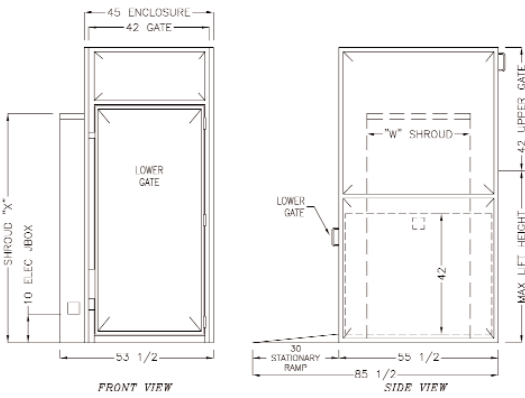
CDE/HCDE Model 2-Gate with Steel Side Guard
