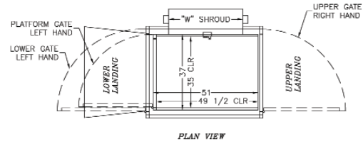
PLAN VIEW
