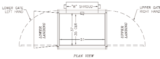
PLAN VIEW
